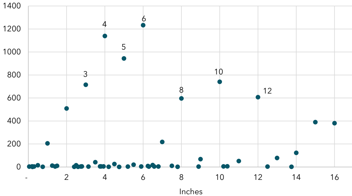
Figure 26. Interior-to-external windowsill depth
