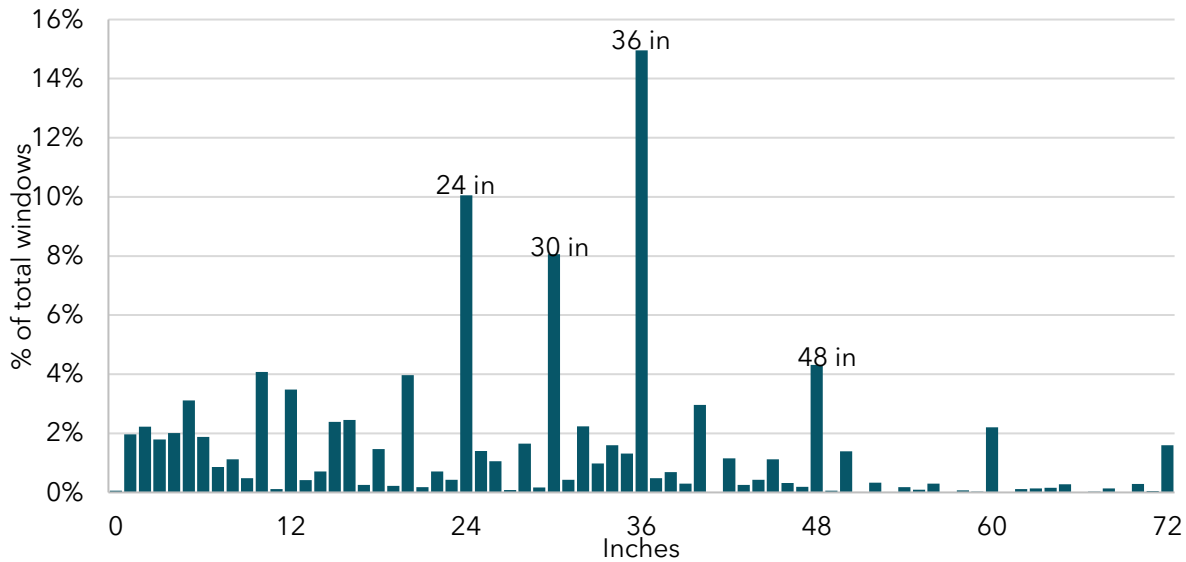
Figure 11. Distribution of window frame-to-floor distances (n=8,266)
